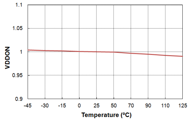
Figure 16. V DD_ON vs. Temperature
