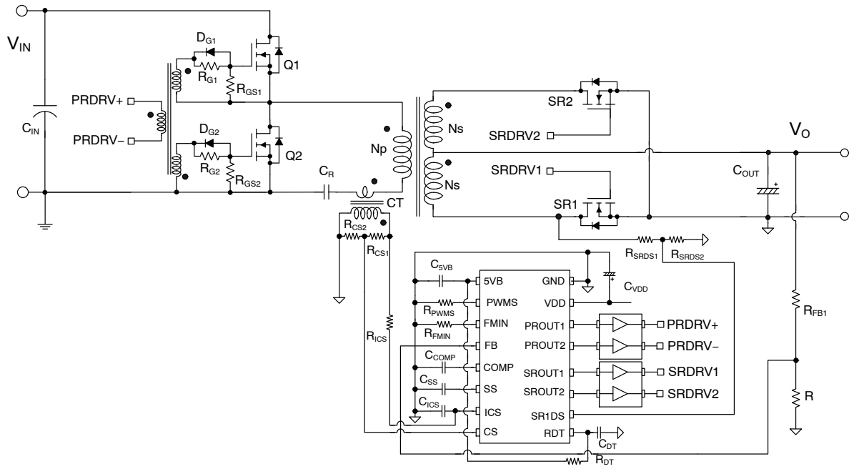
Figure 1. Typical Application Schematic of NCV4390
