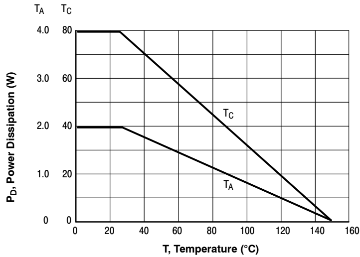
Figure 2. Power Derating
