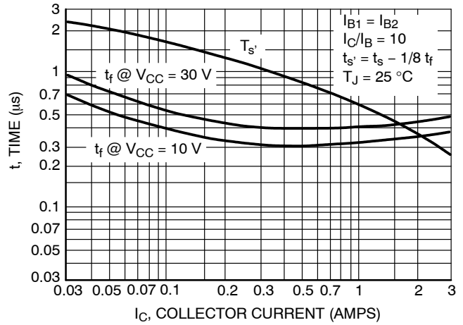
Figure 4. Turn-Off Time
