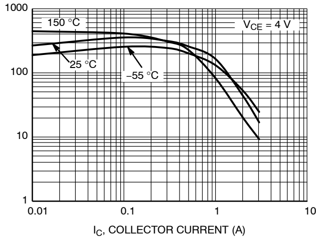
Figure 6. DC Current Gain at V_{CE} = 4\text{ V}
