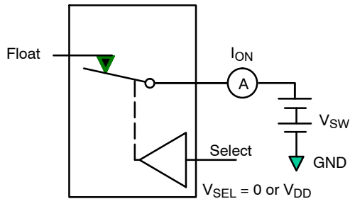
Figure 10. On Leakage
