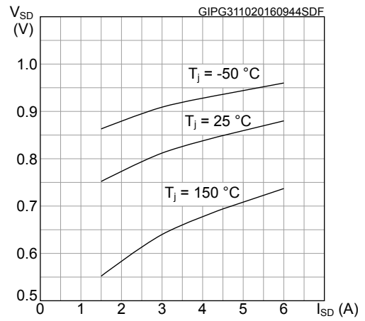
Figure 8. Typical reverse diode forward characteristics
