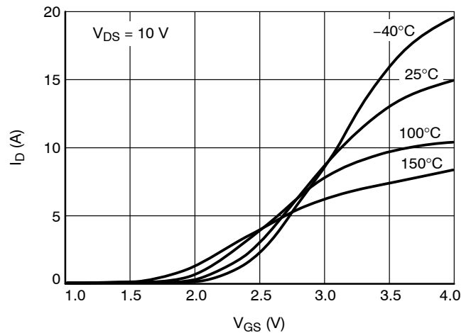
Figure 7. Transfer Characteristics
