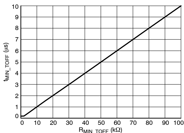
Figure 47. MIN_TOFF Adjust Characteristics
