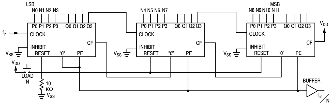
Figure 12. 3 Stages Cascaded
