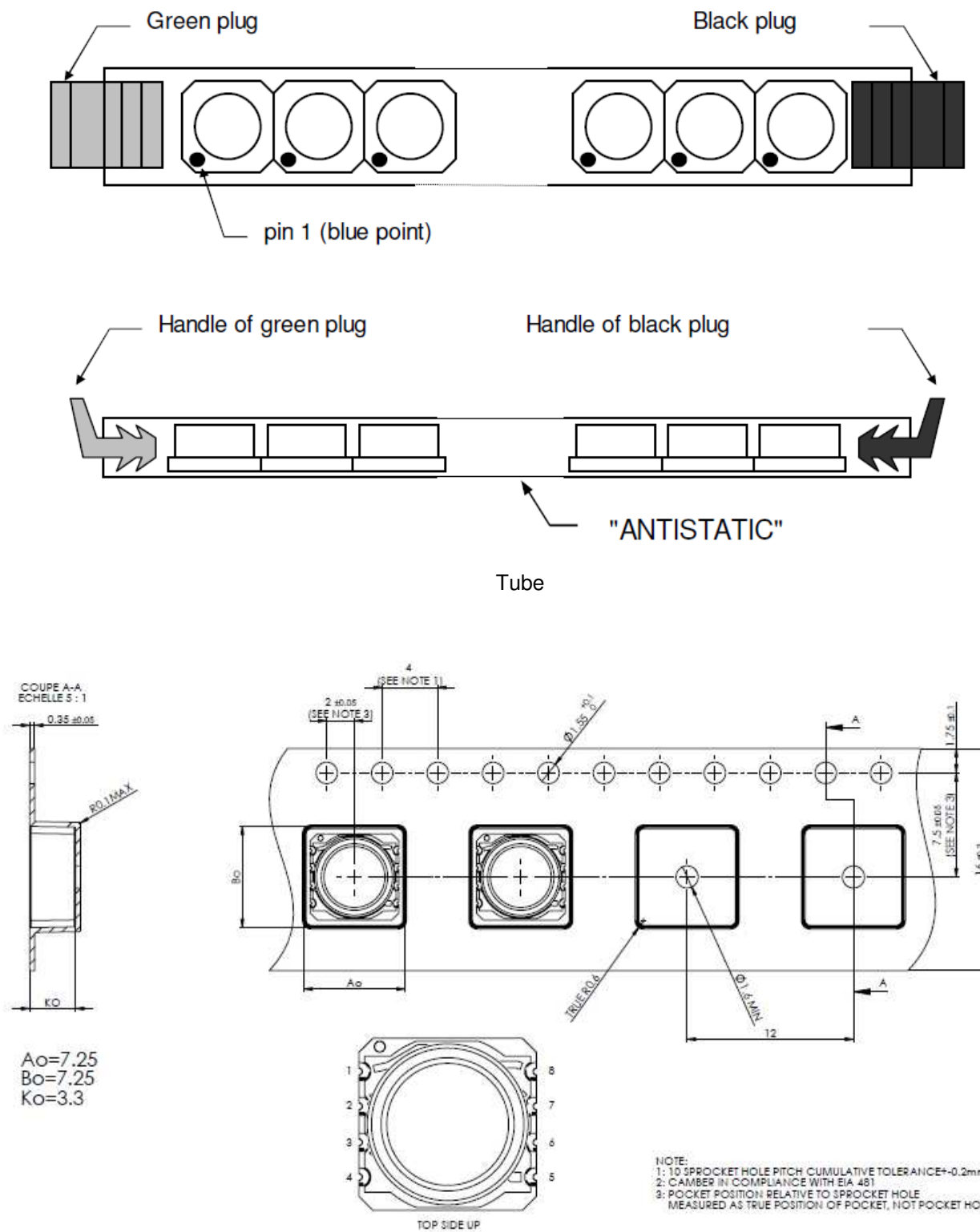
Tape & reel
