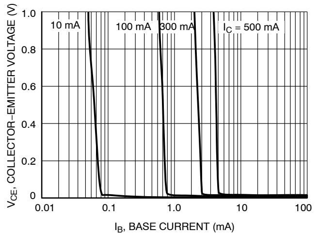
Figure 6. Saturation Region
