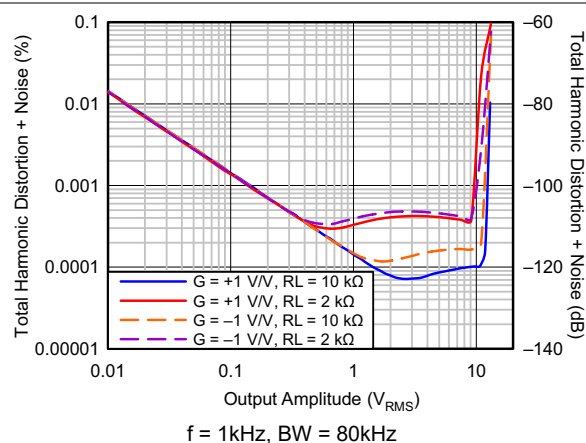
Figure 5-25. THD+N vs Output Amplitude
