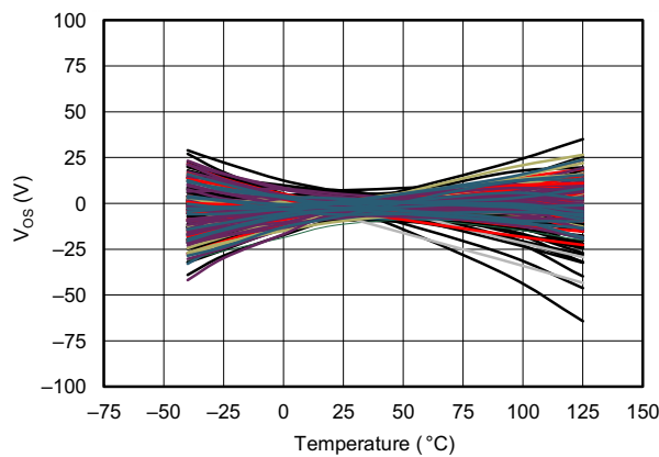
Figure 5-7. Offset Voltage Drift Distribution from -40^\circ\text{C} to +125^\circ\text{C}
