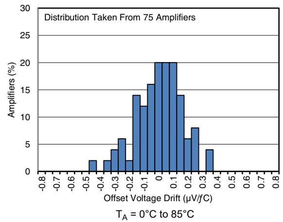
Figure 5-8. Offset Voltage Drift Distribution from 0^\circ\text{C} to 85^\circ\text{C}
