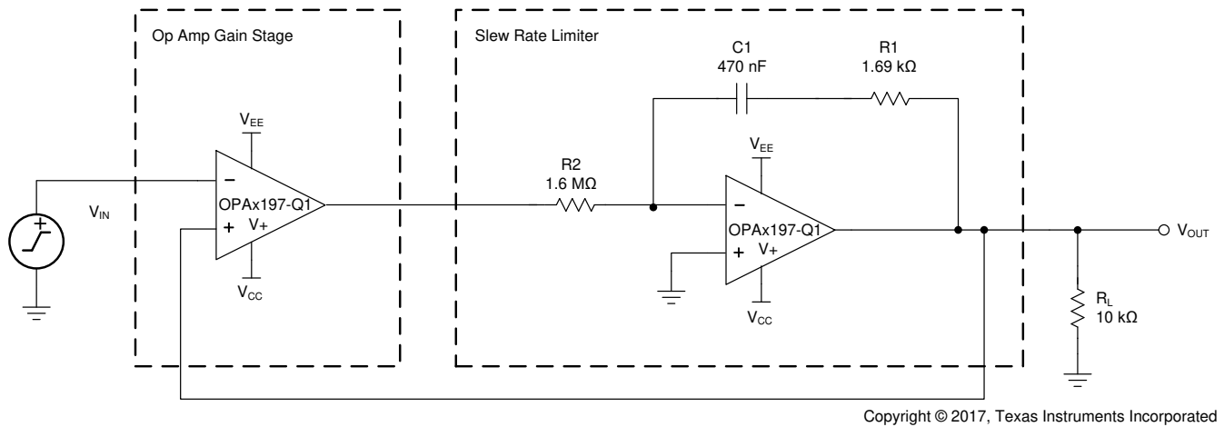
Figure 7-3. Slew-Rate Limiter Uses One Op Amp
