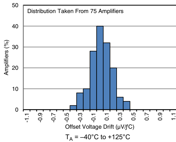
Figure 5-7. Offset Voltage Drift Distribution from -40^\circ\text{C} to +125^\circ\text{C}
