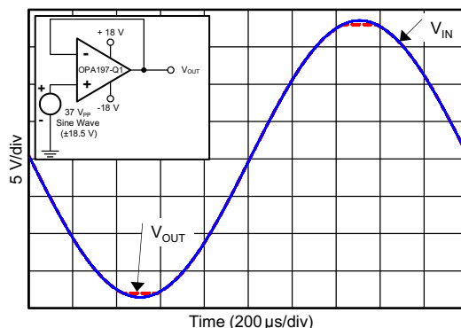
Figure 6-5. No Phase Reversal
