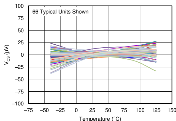
The OPAx197-Q1 Maintains Ultra-Low Input Offset Voltage Over Temperature
