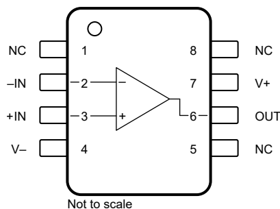
Figure 4-1. OPA197-Q1 DGK Package, 8-Pin VSSOP, Top View
