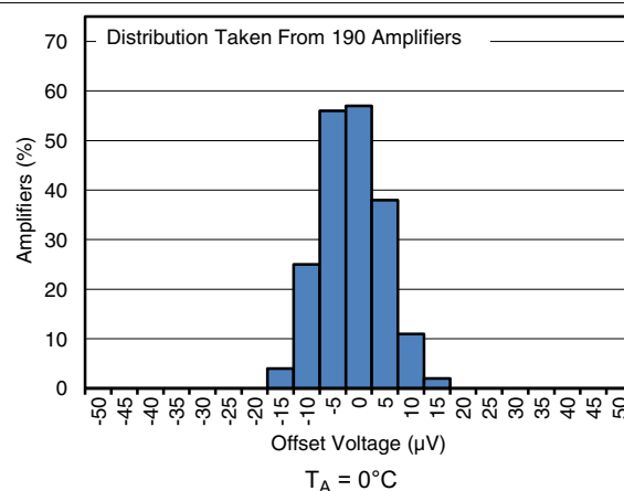
Figure 5-4. Offset Voltage Production Distribution at 0°C
