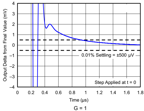
Figure 5-39. Settling Time (5V Positive Step)
