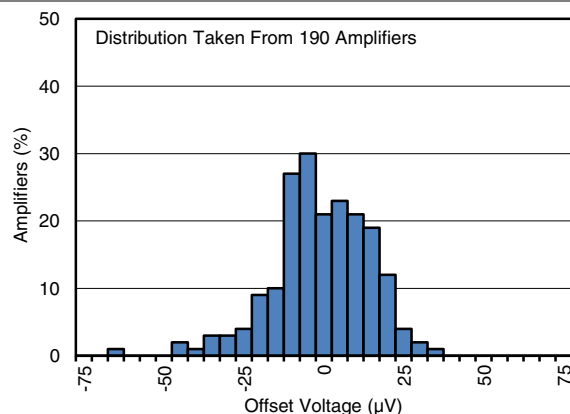
Figure 5-2. Offset Voltage Production Distribution at 125°C
