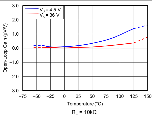
Figure 5-28. Open-Loop Gain vs Temperature
