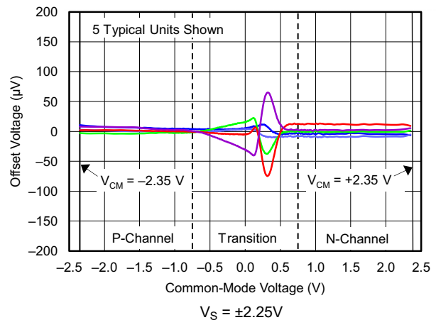
Figure 5-12. Offset Voltage vs Common-Mode Voltage
