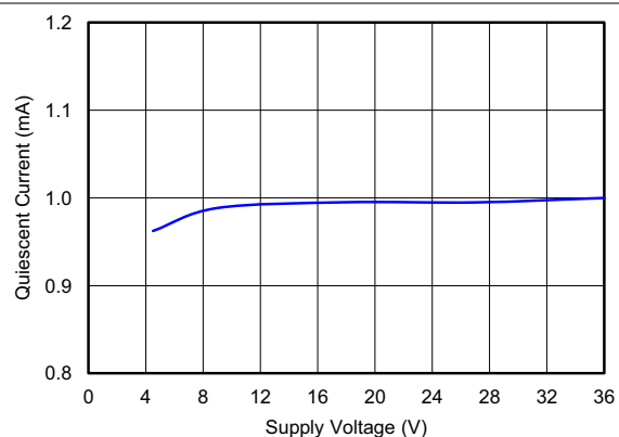
Figure 5-26. Quiescent Current vs Supply Voltage
