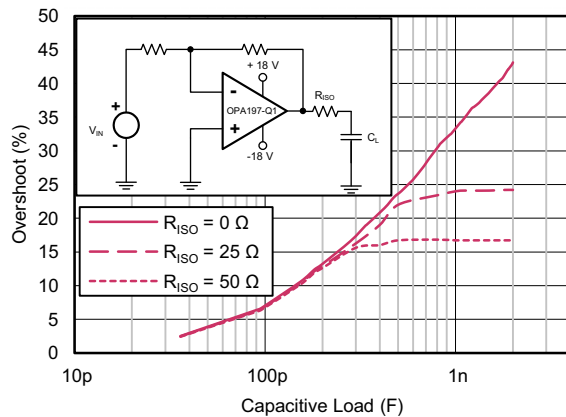
Figure 6-7. Small-Signal Overshoot vs Capacitive Load (100mV Output Step)
