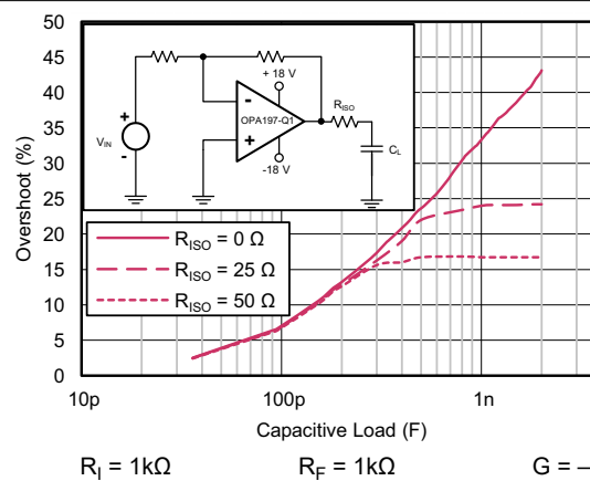
Figure 5-30. Small-Signal Overshoot vs Capacitive Load (100mV Output Step)
