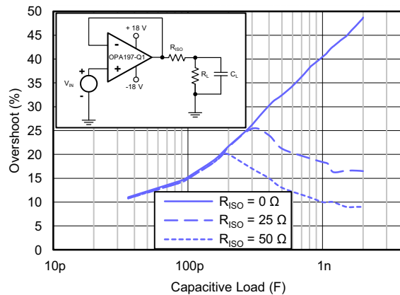
Figure 6-8. Small-Signal Overshoot vs Capacitive Load (100mV Output Step)
