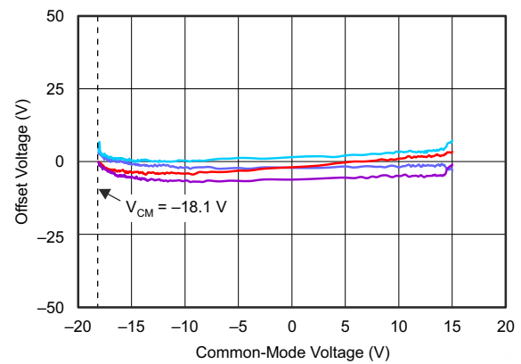
Figure 5-10. Offset Voltage vs Common-Mode Voltage
