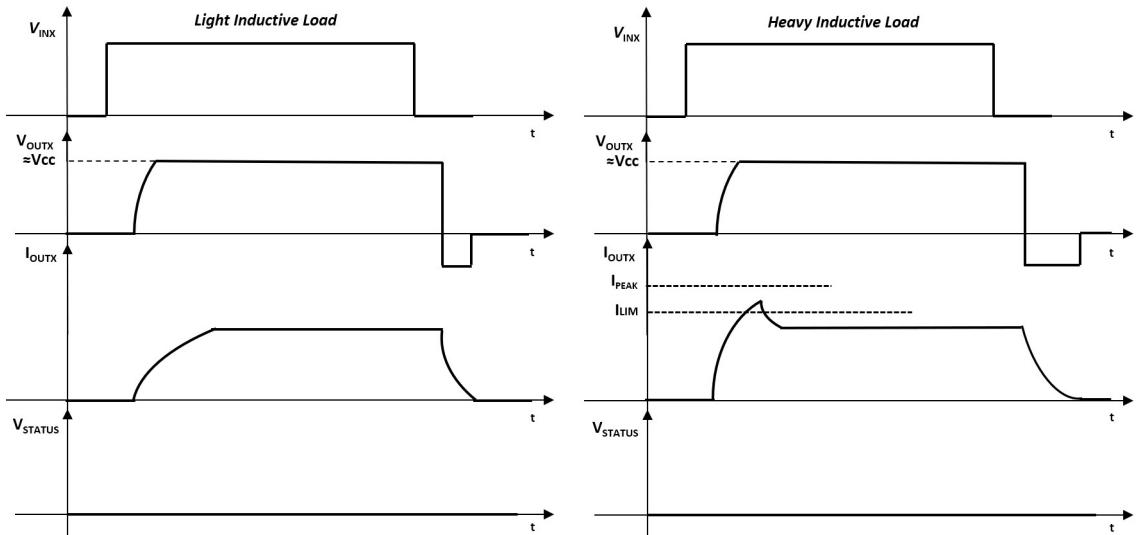
Figure 7. Switching on light and heavy inductive load
