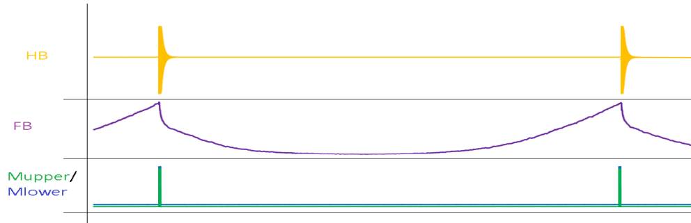
Figure 18. No-load Operation
