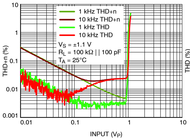
Figure 23. Harmonic Distortion
