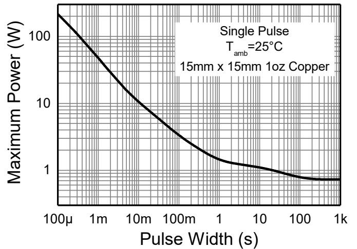
Fig. 4 Pulse Power Dissipation
