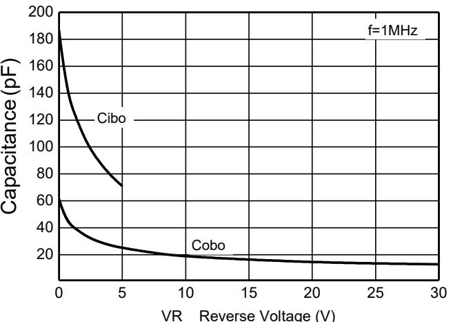
Fig. 10 Typical Junction Capacitance
