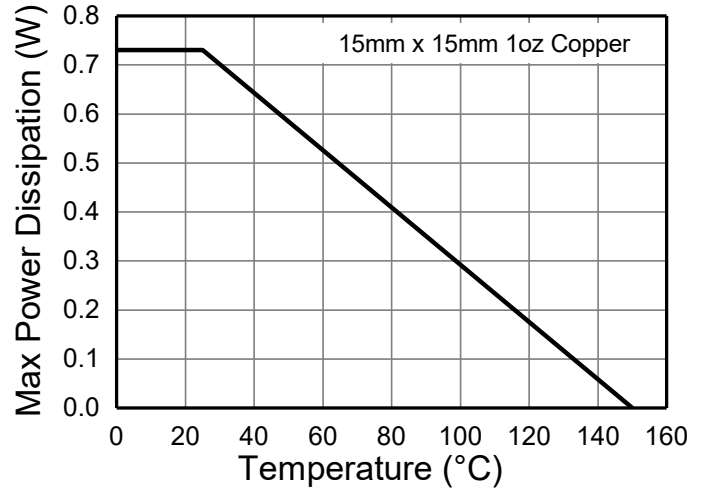
Fig. 2 Derating Curve
