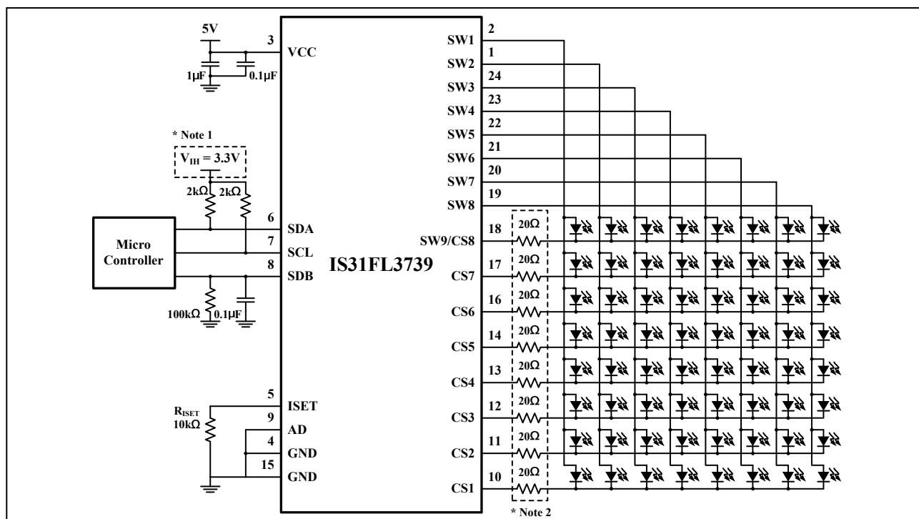
Figure 1 Typical Application Circuit (8×8)
