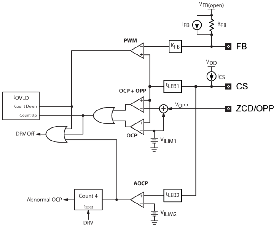
Figure 30. Overload Circuitry
