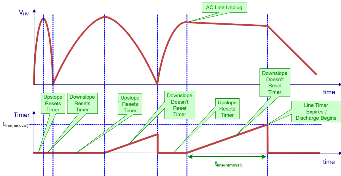
Figure 25. Line Removal Detection Timing
