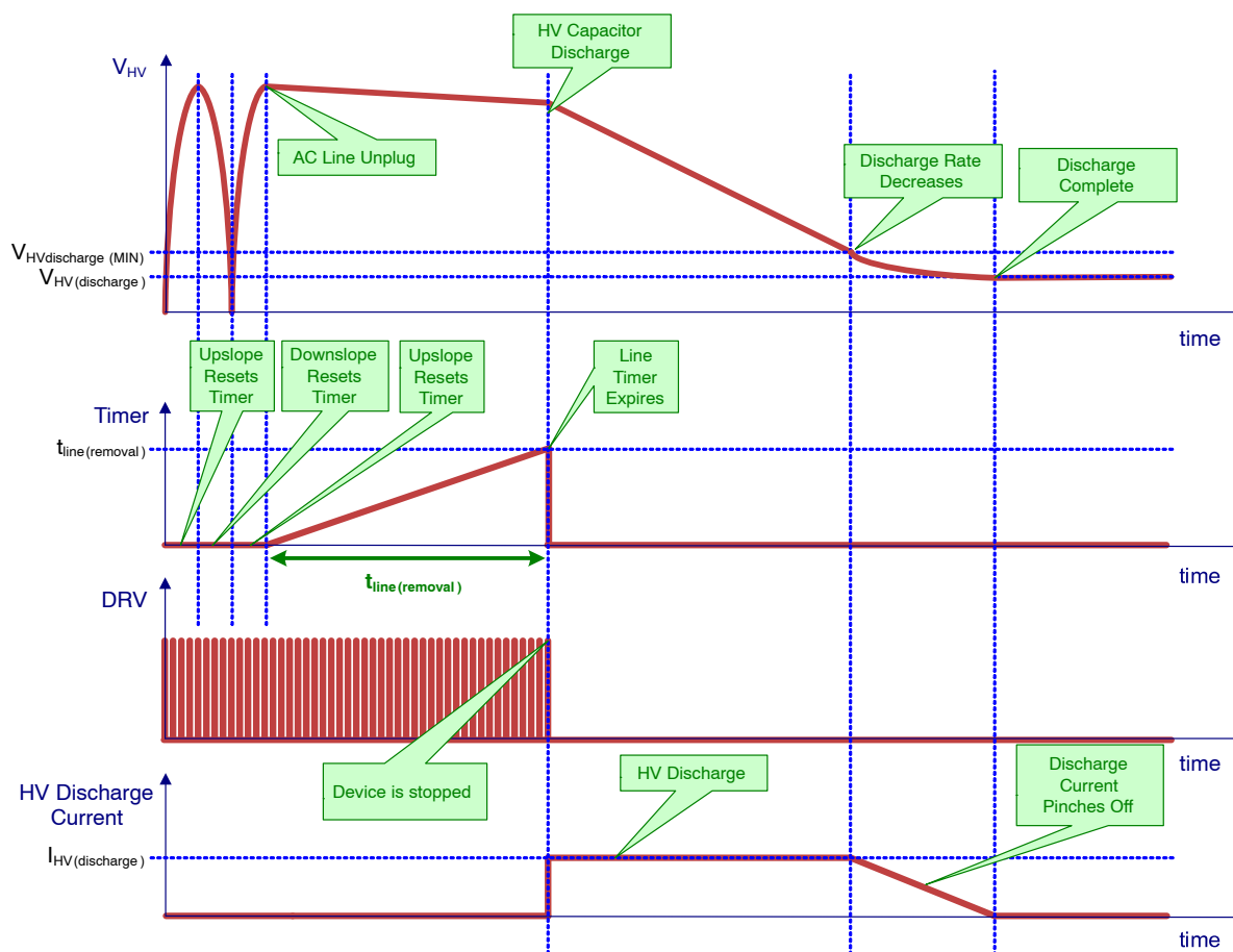
Figure 26. HV Discharge Timing
