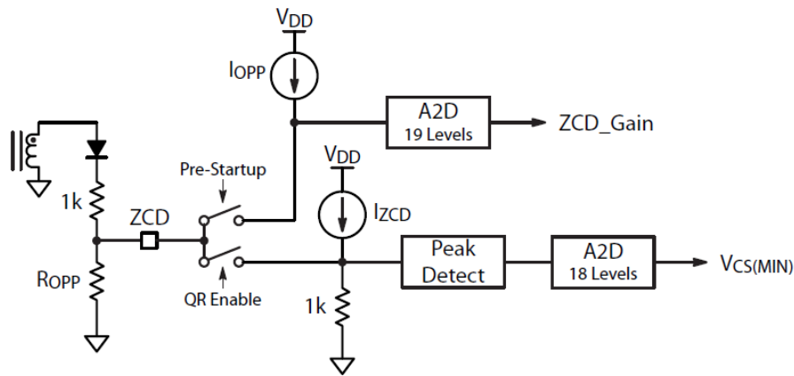
Figure 29. OPP Programming Block
