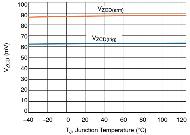
Figure 45. V ZCD(arm/trig) vs. Temperature
