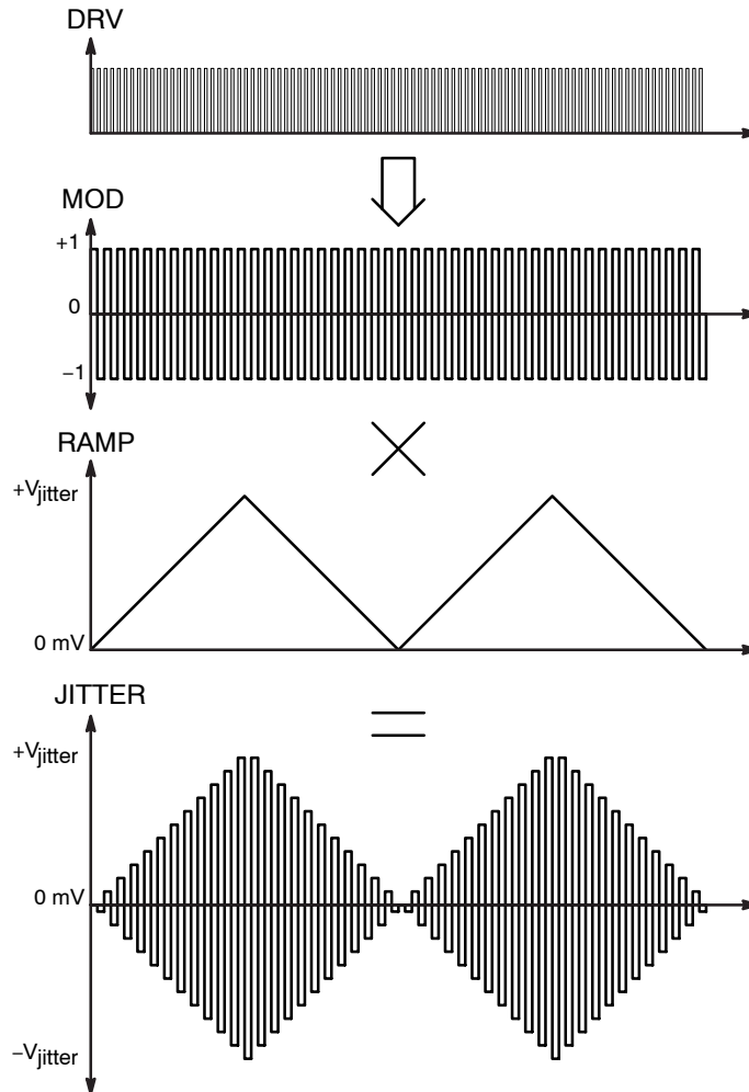
Figure 11. Jitter Timing
