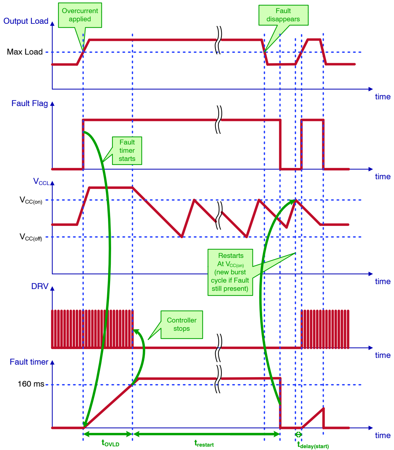
Figure 32. Auto-Recovery Overload Operation
