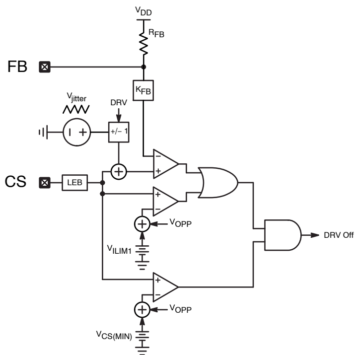
Figure 12. Jitter Implementation
