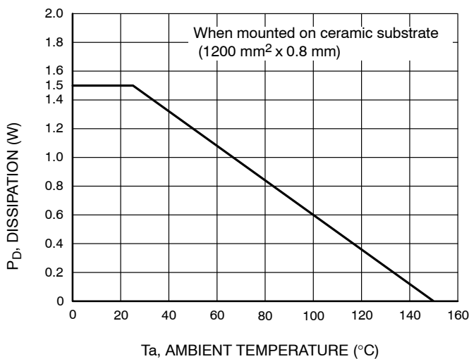
Figure 12. P_D – T_a
