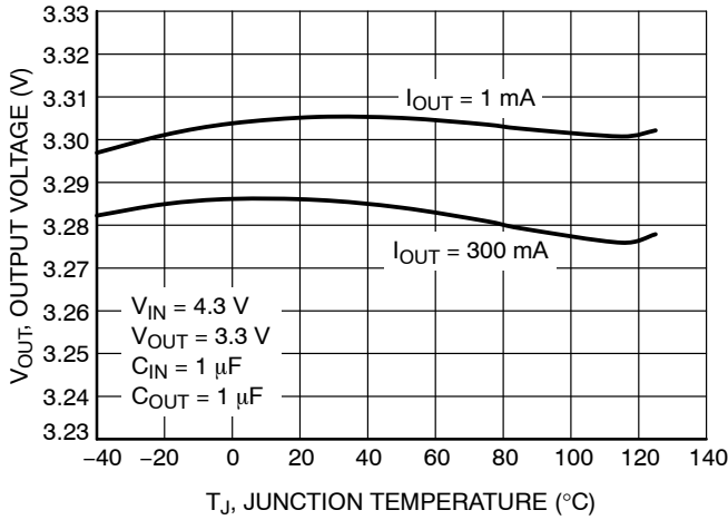
Figure 3. Output Voltage vs. Temperature – V_{OUT} = 3.3\text{ V}
