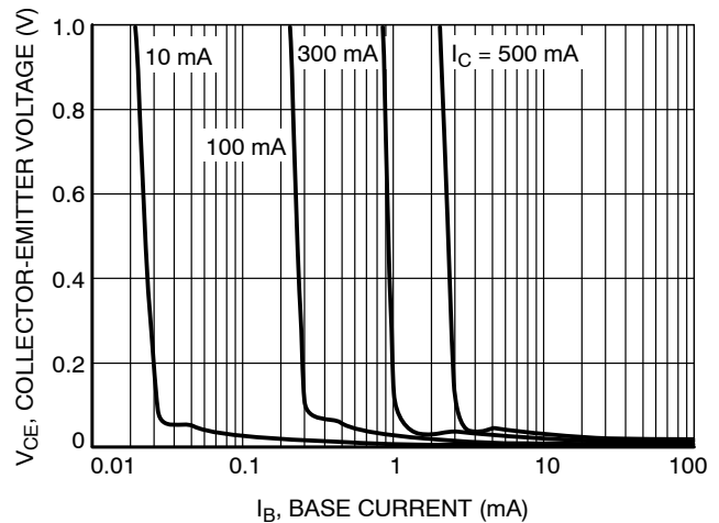
Figure 6. Saturation Region
