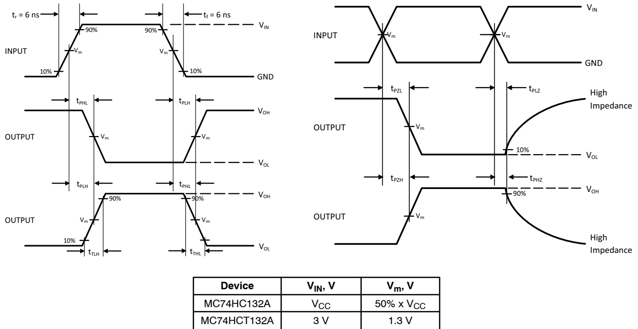
Figure 3. Switching Waveforms
