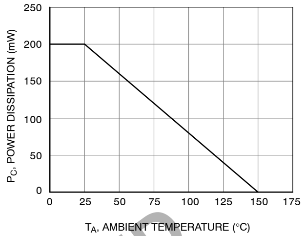
Figure 8. Power Derating
