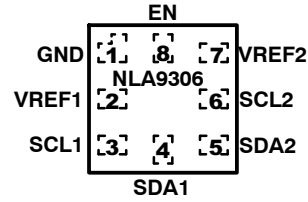
Figure 3. UQFN8 Pinout (Top Thru View)
