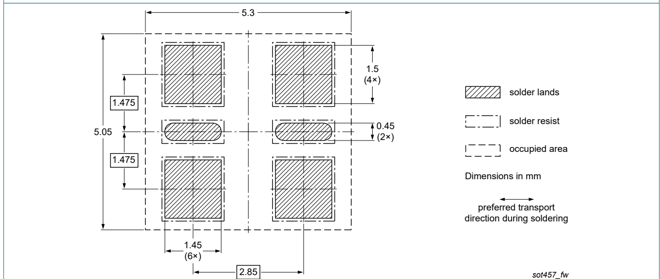
Fig. 13. Wave soldering footprint for TSOP6 (SOT457)
