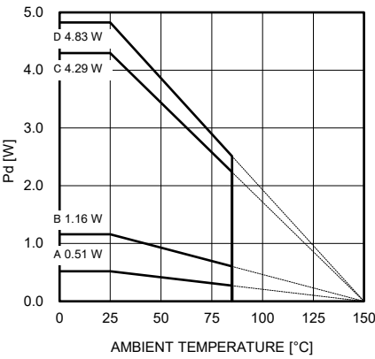
Figure 35. Thermal Derating Curve (VQFN048V7070)
