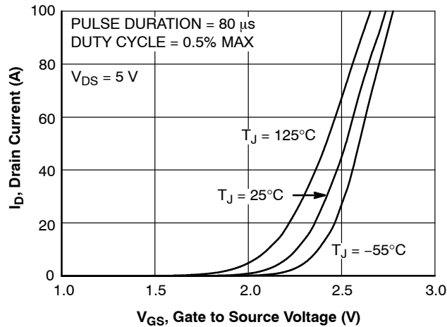
Figure 18. Transfer Characteristics
