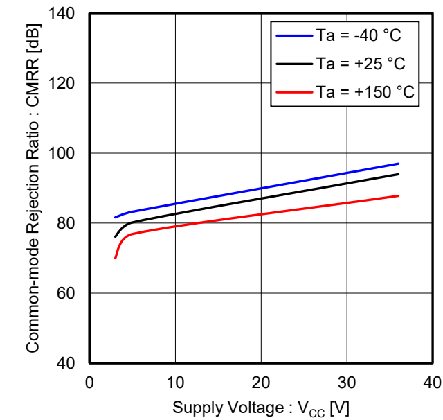
Figure 21. Common-mode Rejection Ratio vs Supply Voltage (V OUT = 1.4 V)
