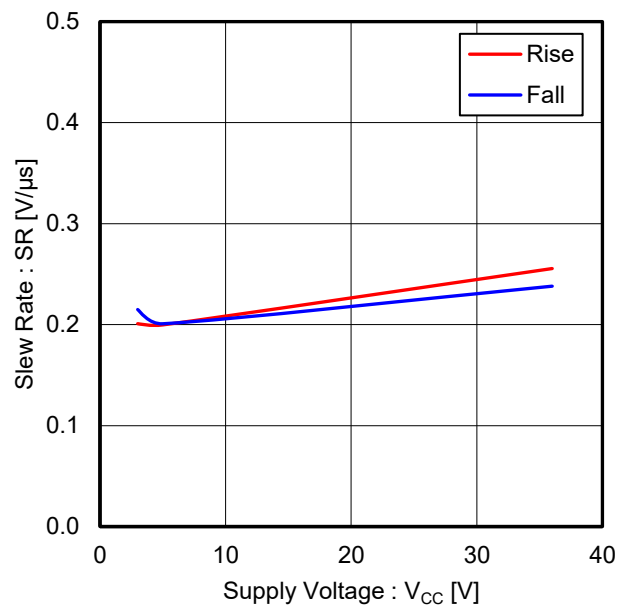
Figure 24. Slew Rate vs Supply Voltage (Ta = 25 °C, R L = 2 kΩ)
