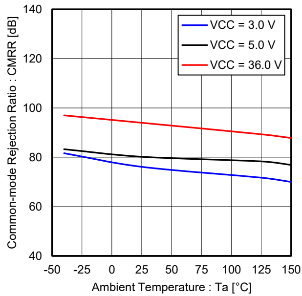
Figure 22. Common-mode Rejection Ratio vs Ambient Temperature (V OUT = 1.4 V)
