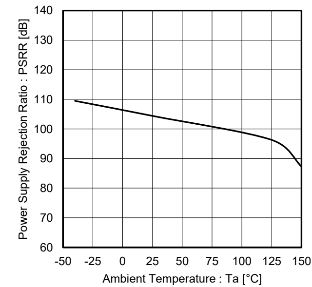
Figure 23. Power Supply Rejection Ratio vs Ambient Temperature (V CC = 5 V)
