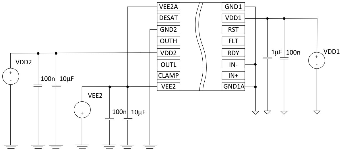
Figure 24. Bipolar Power Supply
