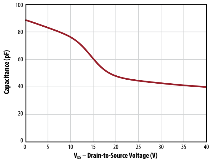
Figure 6: Typical C_{oss}
