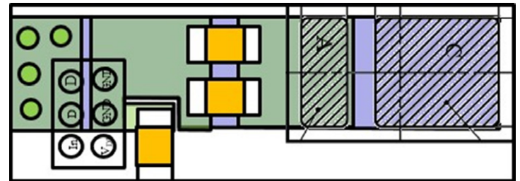
Figure 10: Recommended Layout
