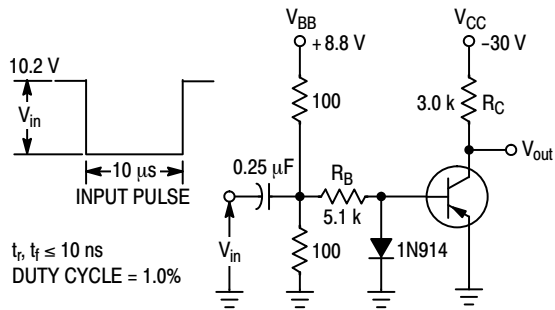
Figure 8. Switching Time Test Circuit
