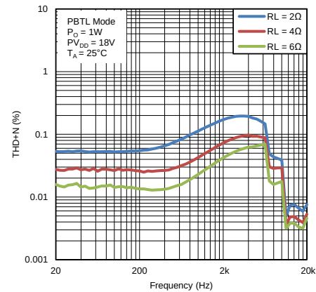
Figure 38. Total Harmonic Distortion + Noise vs Frequency (PBTL Mode)
