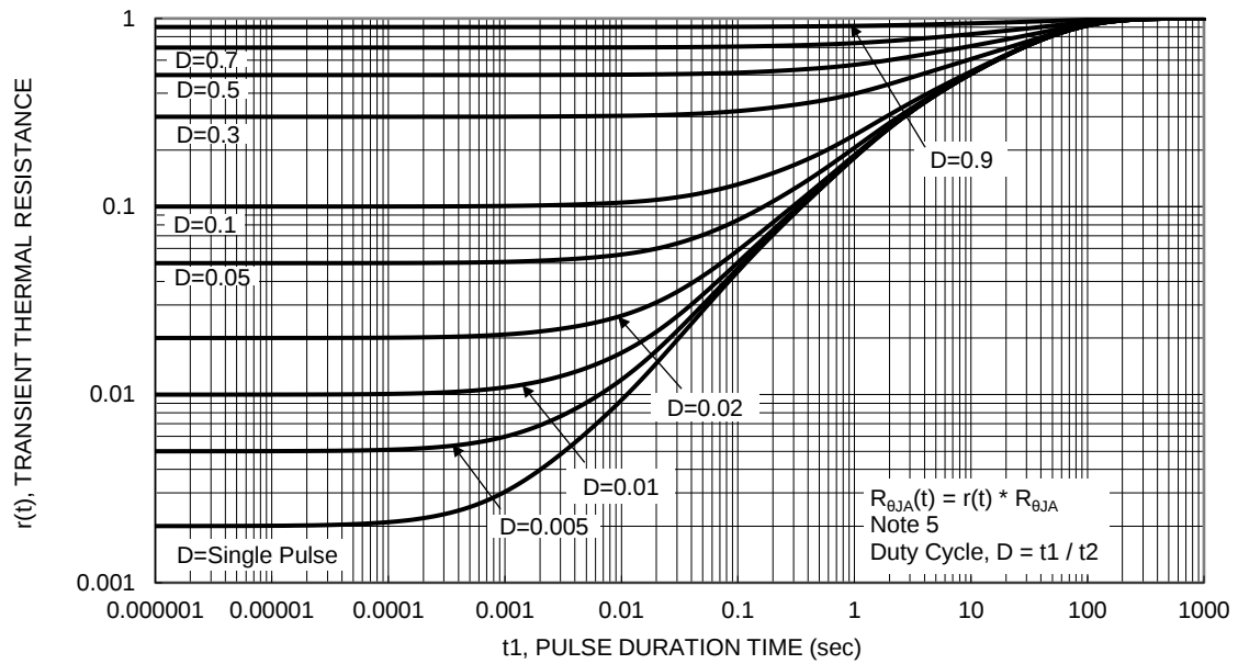
Figure 9 Transient Thermal Resistance
