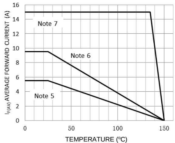
Figure 6 Forward Current Derating Curve D = 1
