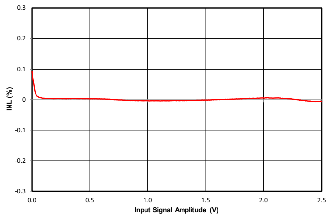
Figure 10. Si8932 Nonlinearity (%) vs. Input Signal Amplitude (mV)
