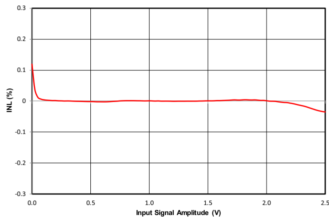
Figure 9. Si8931 Nonlinearity (%) vs. Input Signal Amplitude (mV)
