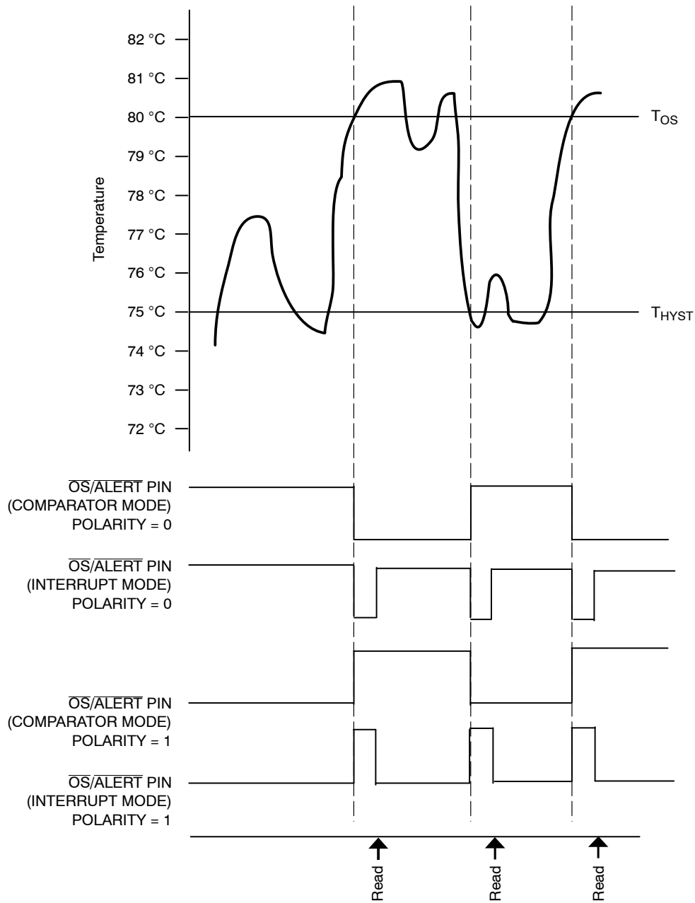
Figure 11. \overline{\text{OS}}/\text{ALERT} Output Temperature Response Diagram
