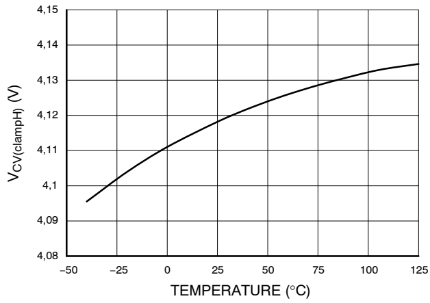
Figure 35. V CV(clampH) vs. Temperature
