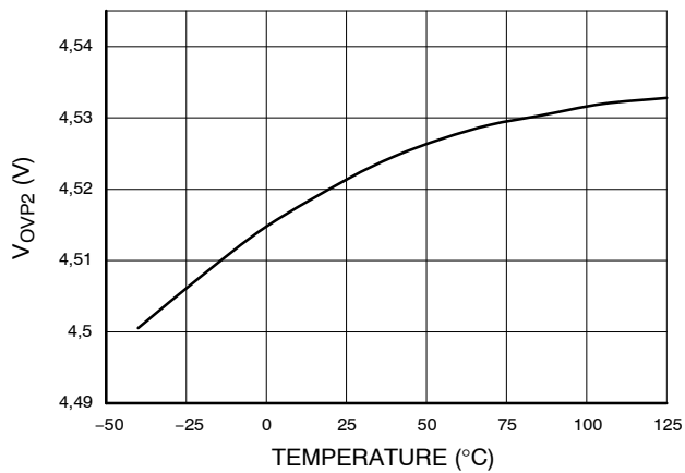
Figure 37. V OVP2 vs. Temperature
