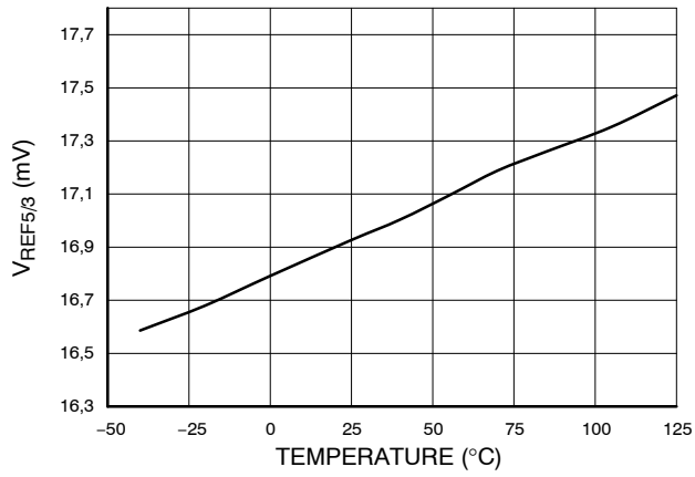
Figure 33. V REF5/3 vs. Temperature
