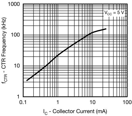
Fig. 12 - CTR Frequency vs. Collector Current
