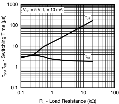
Fig. 13 - Switching Time vs. Load Resistance
