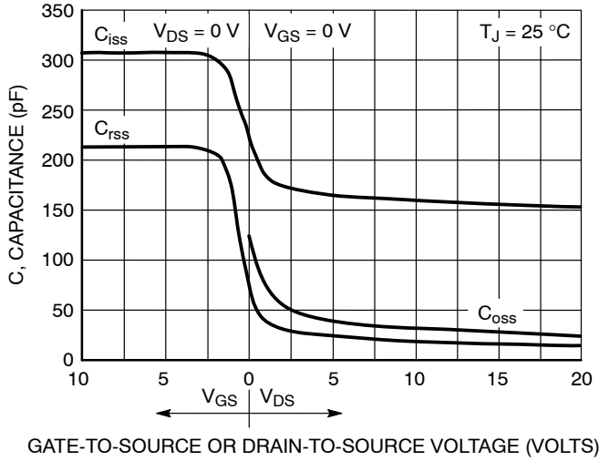
Figure 11. Capacitance Variation
