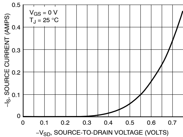
Figure 14. Diode Forward Voltage vs. Current
