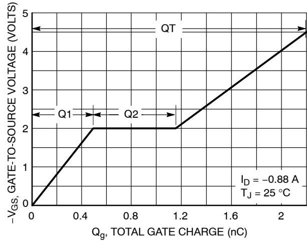
Figure 12. Gate-to-Source Voltage vs. Total Gate Charge
