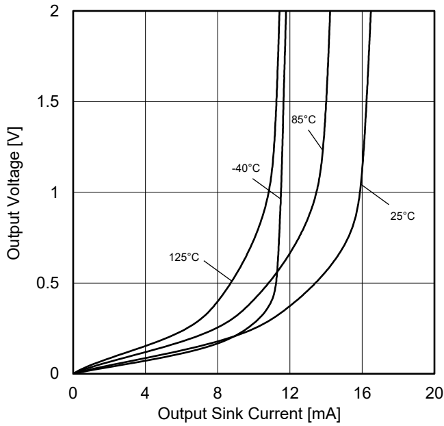
Figure 24. Output Voltage vs Output Sink Current (V CC =5V)
