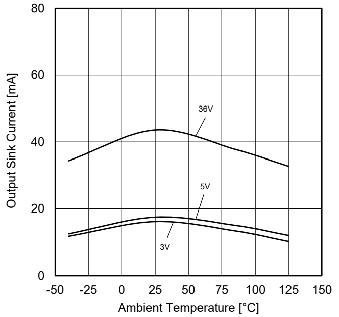
Figure 25. Output Sink Current vs Ambient Temperature (V OUT =V CC )
