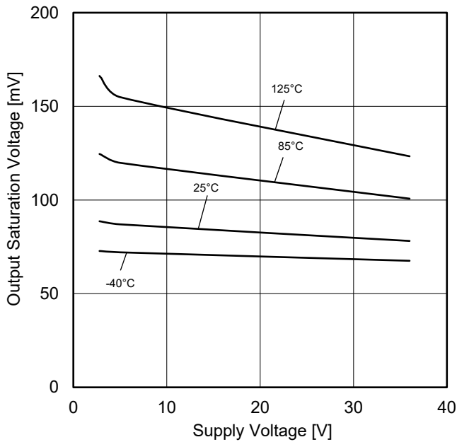
Figure 3. Output Saturation Voltage vs Supply Voltage (I SINK =4mA)
