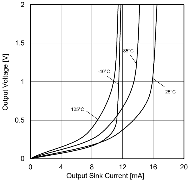
Figure 5. Output Voltage vs Output Sink Current (V CC =5V)
