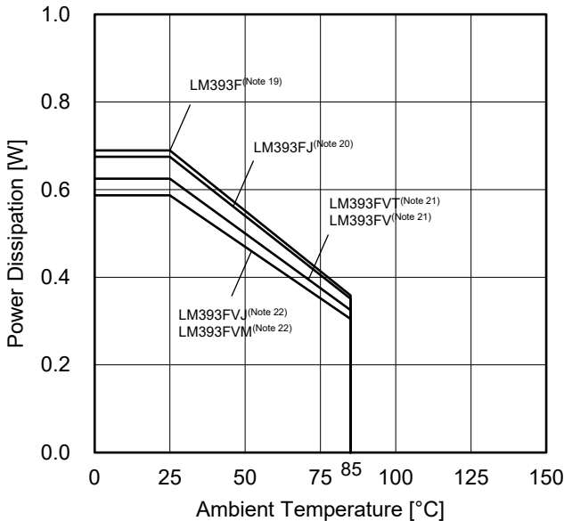
(c) LM393xxx*1
