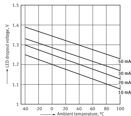
4. LED dropout voltage vs. ambient temperature characteristics
