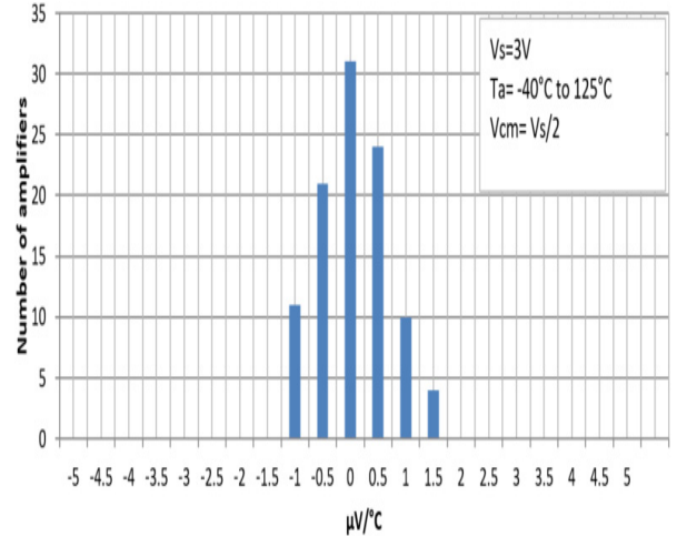
Figure 4. Input Offset Voltage vs. Temperature Distribution, V_S = 3\text{ V}
