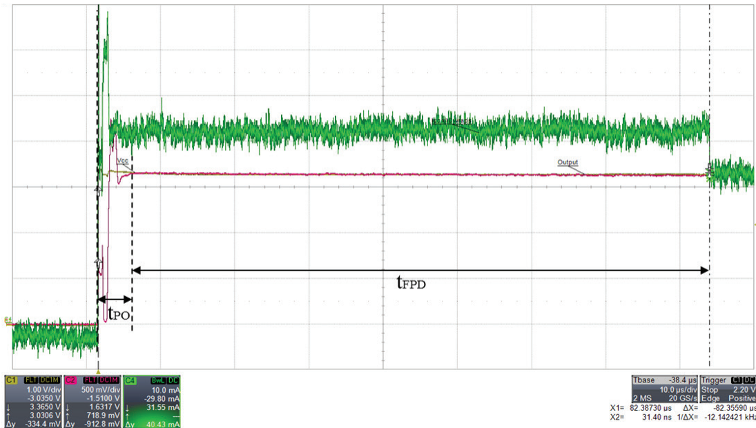
Figure 5: Power-On Behavior
