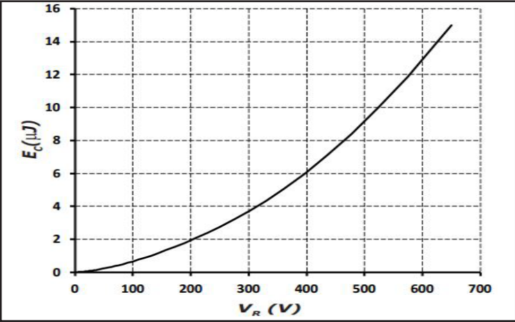
Figure 7 Capacitance Stored Energy
