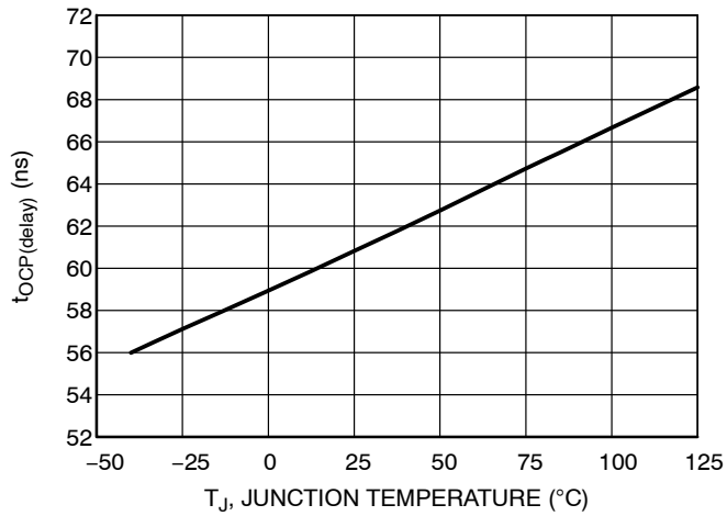
Figure 52. t OCP(delay) vs. Temperature
