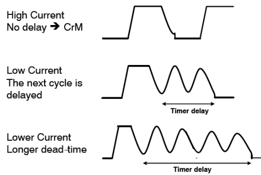
Figure 3. CCFF Operation
