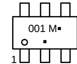
TSOT23 6-Lead CASE 419BL
