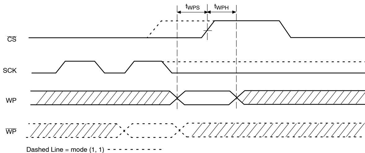
Figure 8. \overline{WP} Timing
