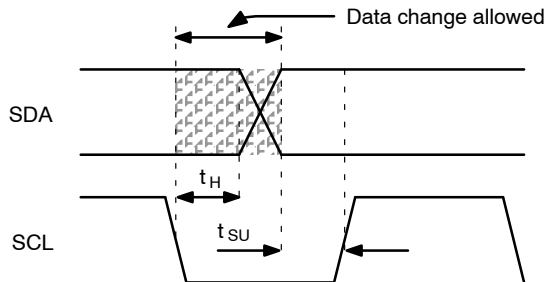
Figure 13. Data Transfer Timing
