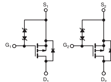
Dual P-Channel MOSFET
