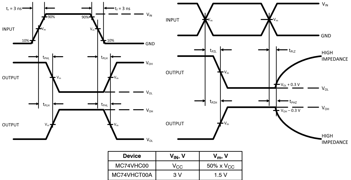
Figure 2. Switching Waveforms
