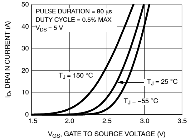
Figure 6. Transfer Characteristics
