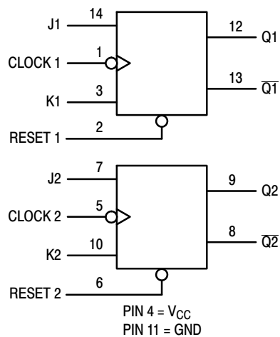
Figure 1. Logic Diagram
